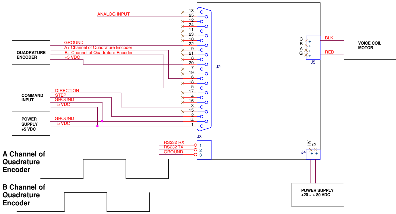
Encoder Phase Relationship when the Motor Is Moving Outward.
